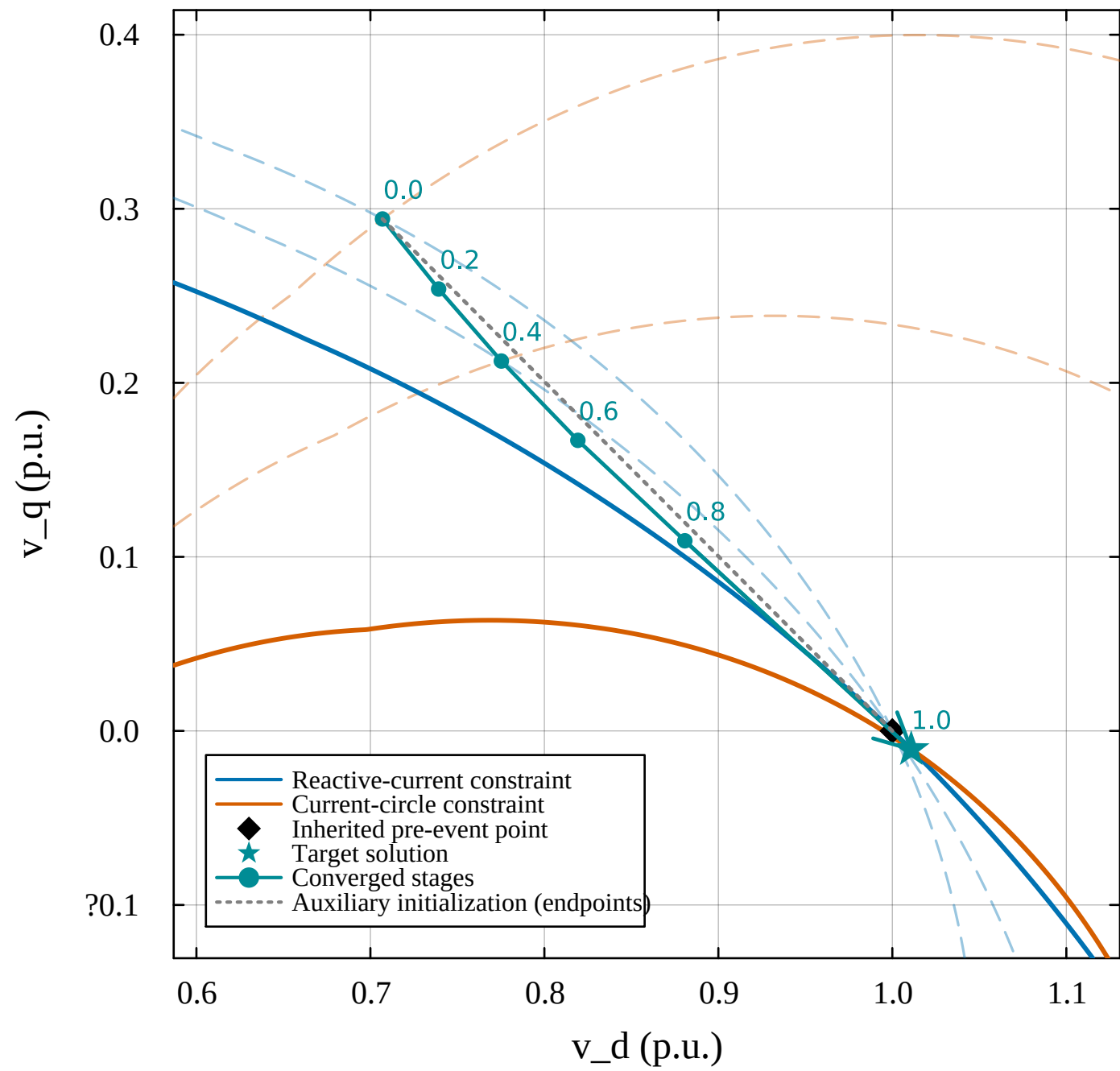
(b) Continuation solutions
