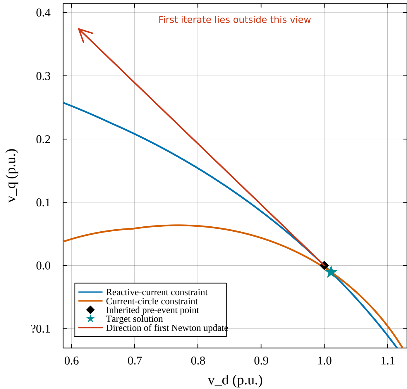
(a) Direct Newton: voltage projection
