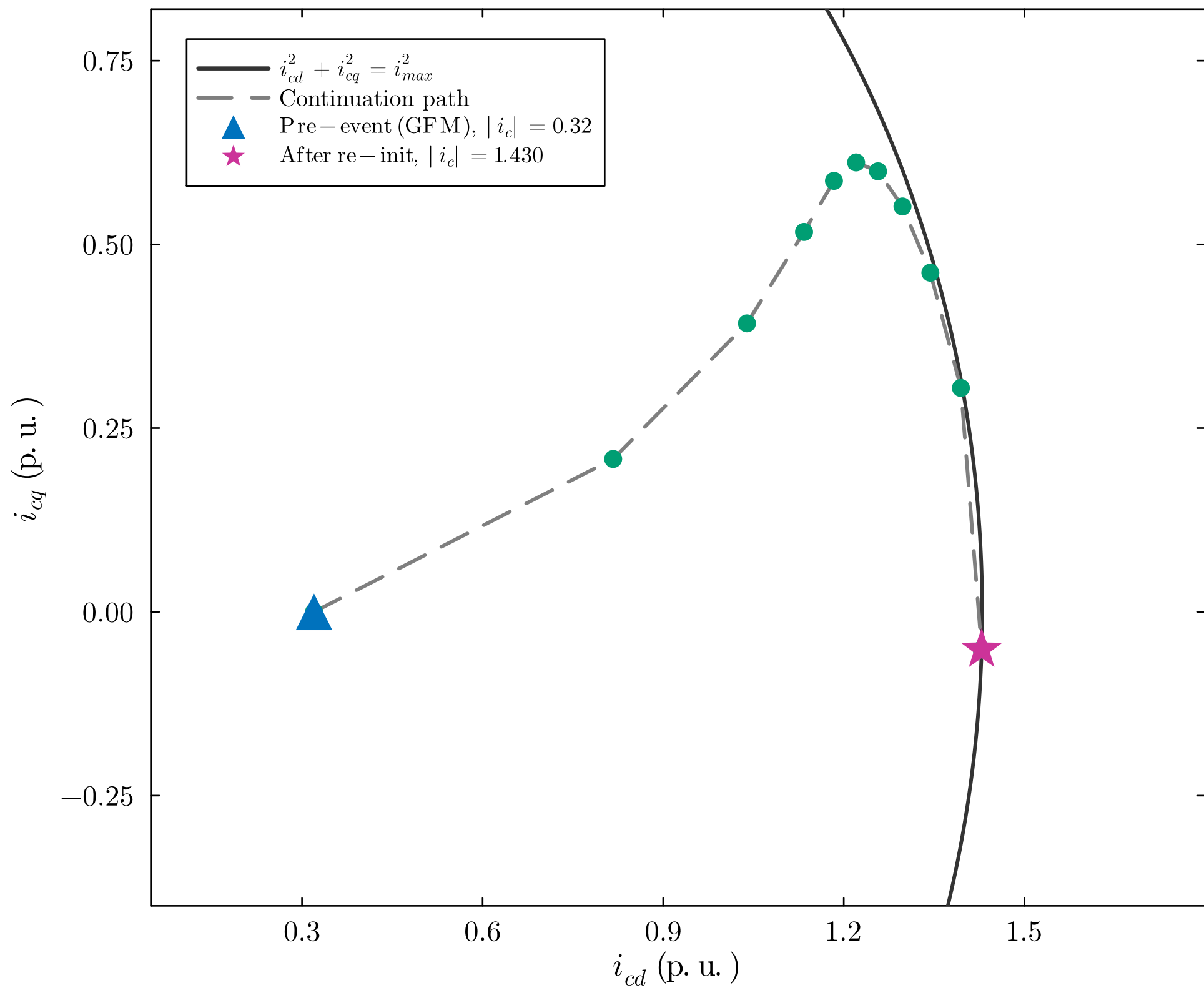
(a) Converter current plane
