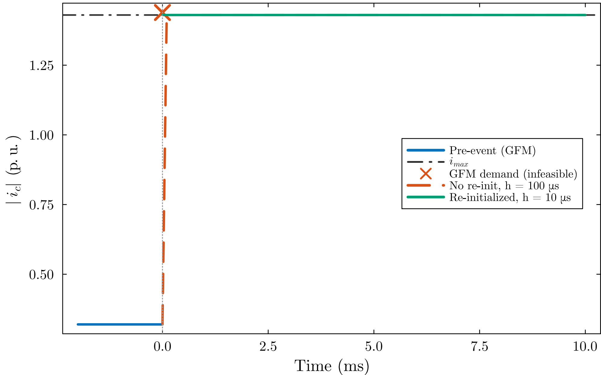
(e) Converter current magnitude
