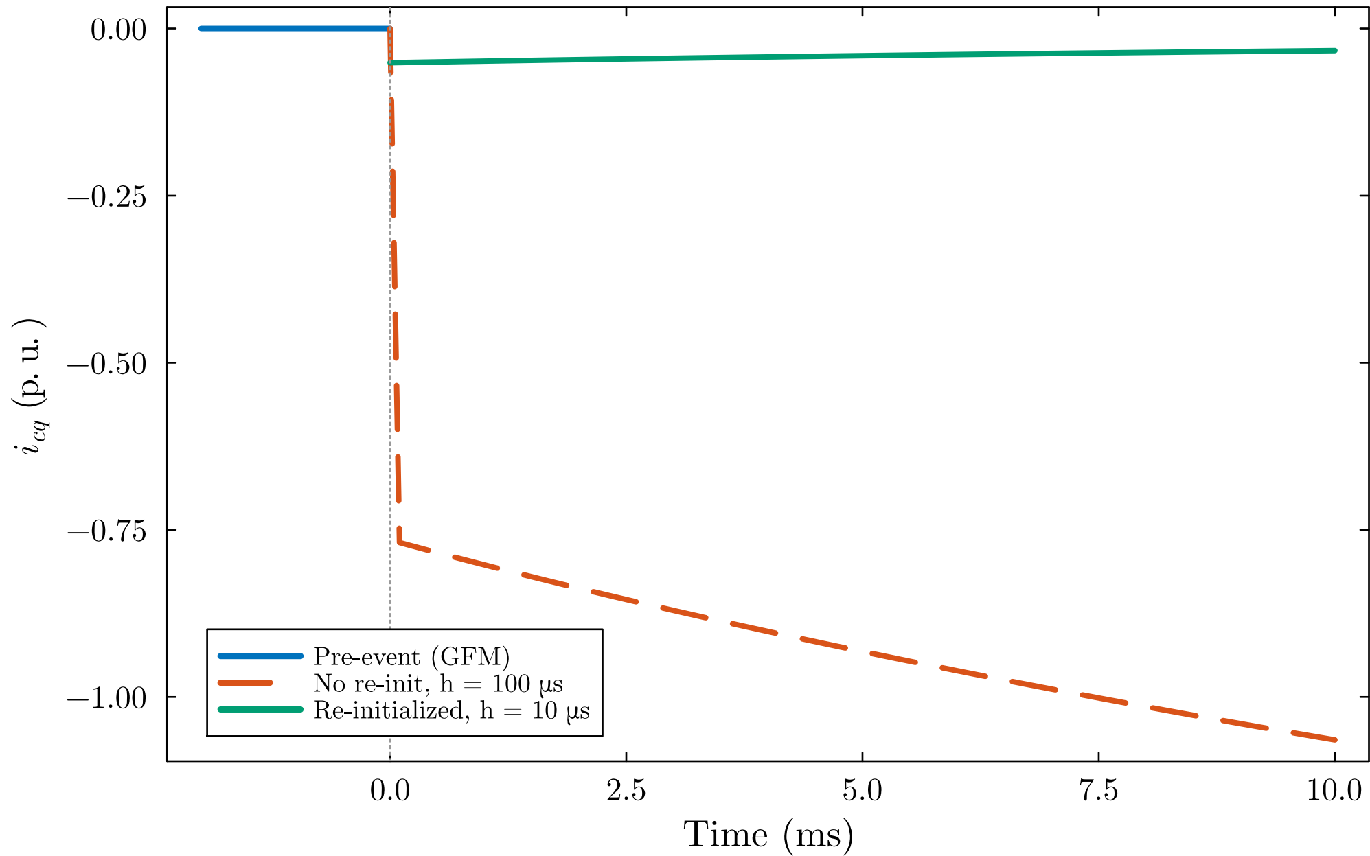
(f) Converter q-axis current
