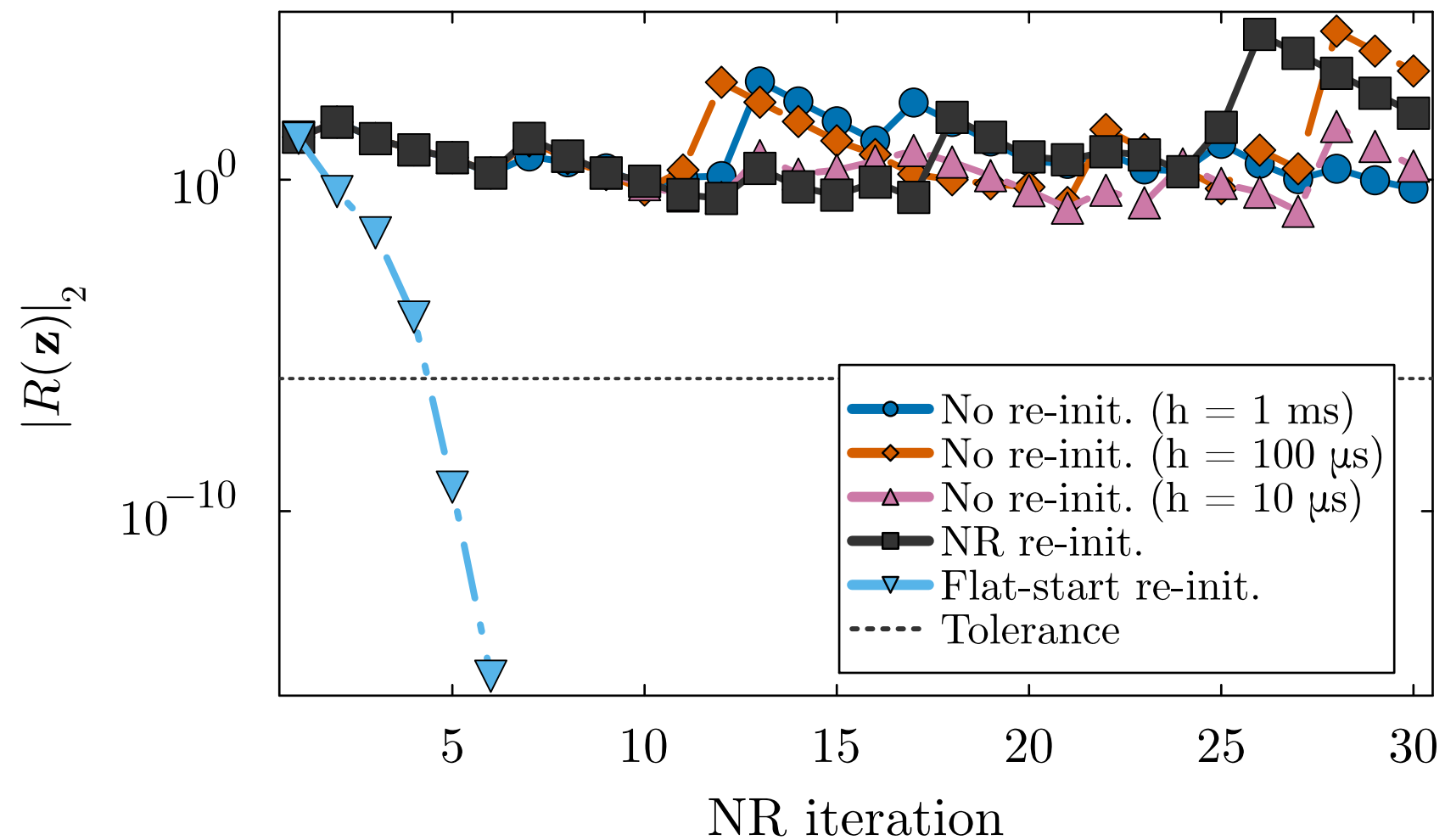
(b) Newton residual
