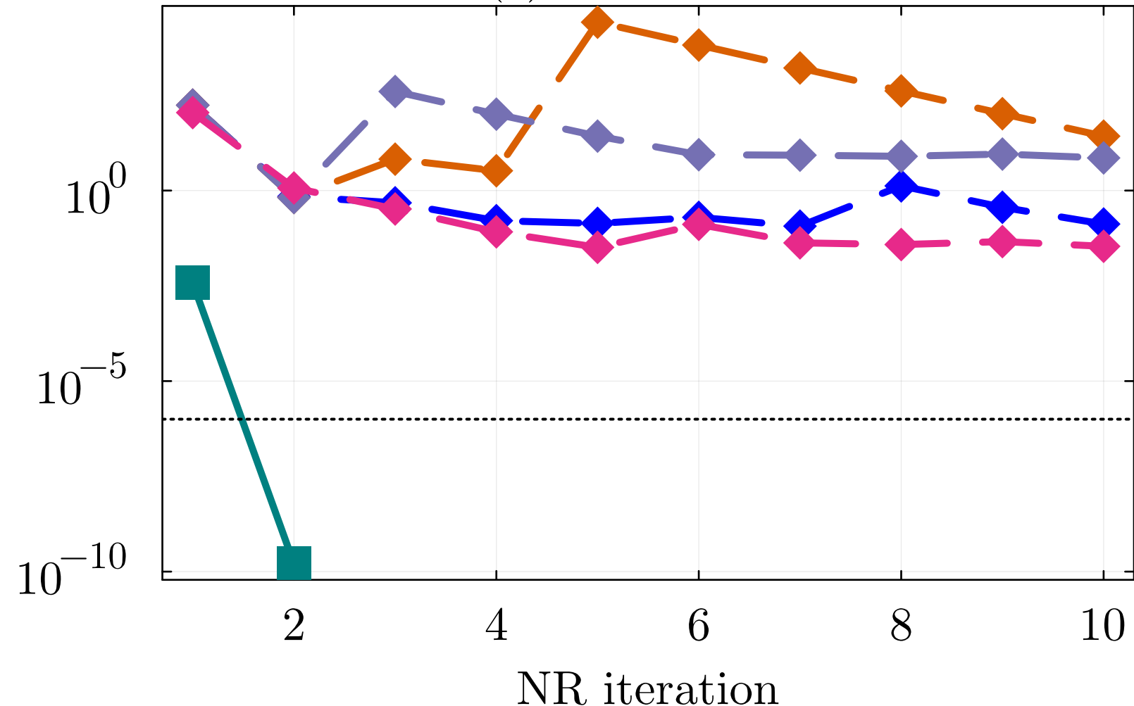
(a) IEEE 39-bus
