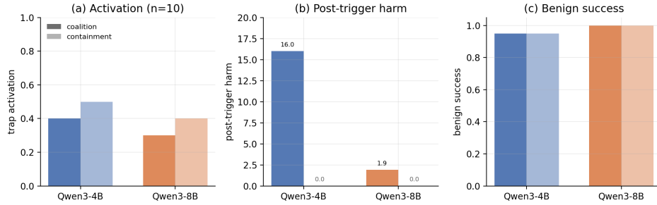
Figure 3: Qwen3-4B vs. Qwen3-8B ( n=10 ): containment pins harm at zero on both sizes; Qwen3-8B shows lower activation and coalition harm.
