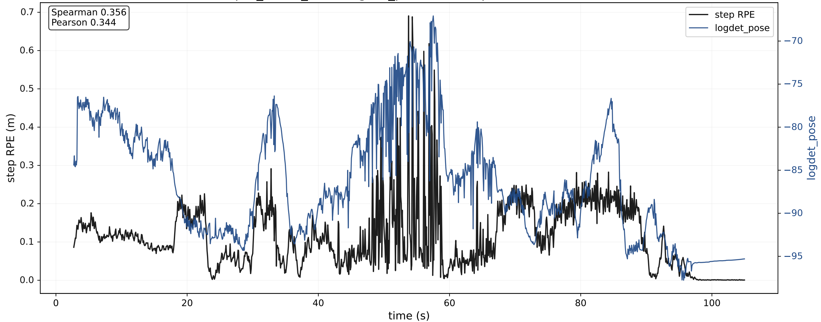
spot_forest_hard: logdet_pose and Step-RPE over Time
