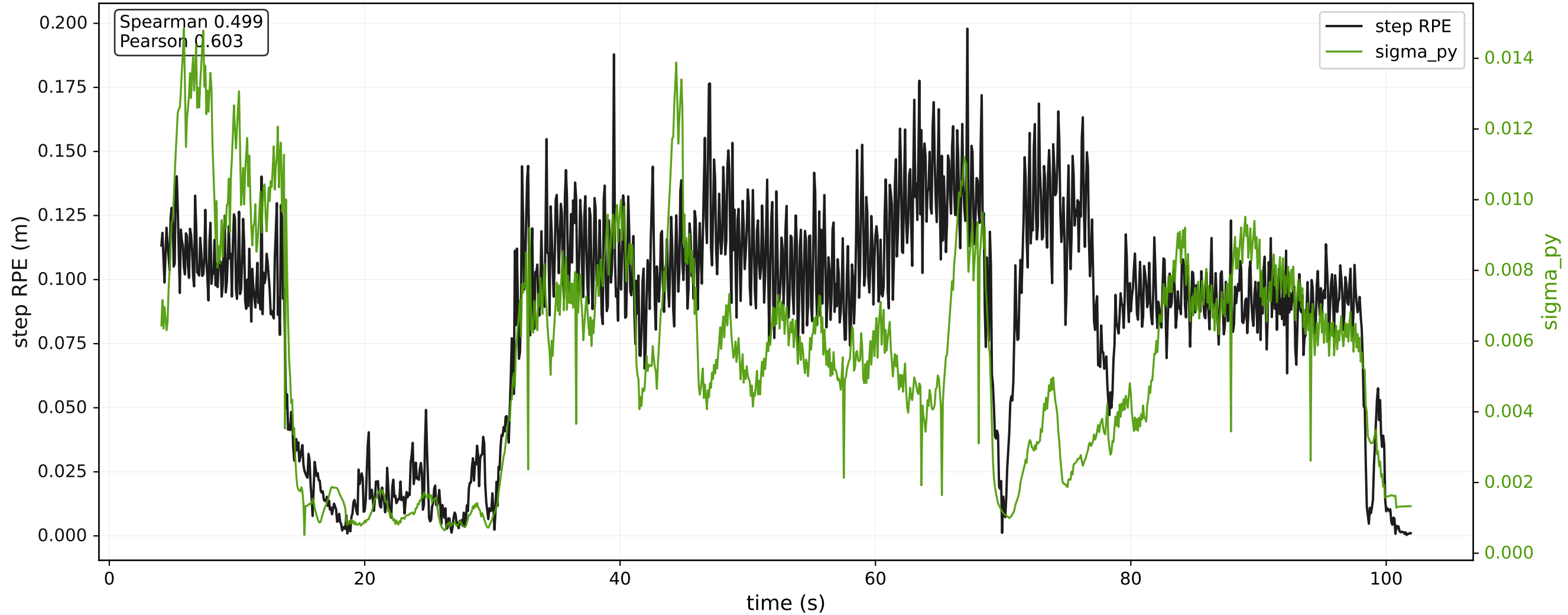
spot_indoor_building_loop: sigma_py and Step-RPE over Time
