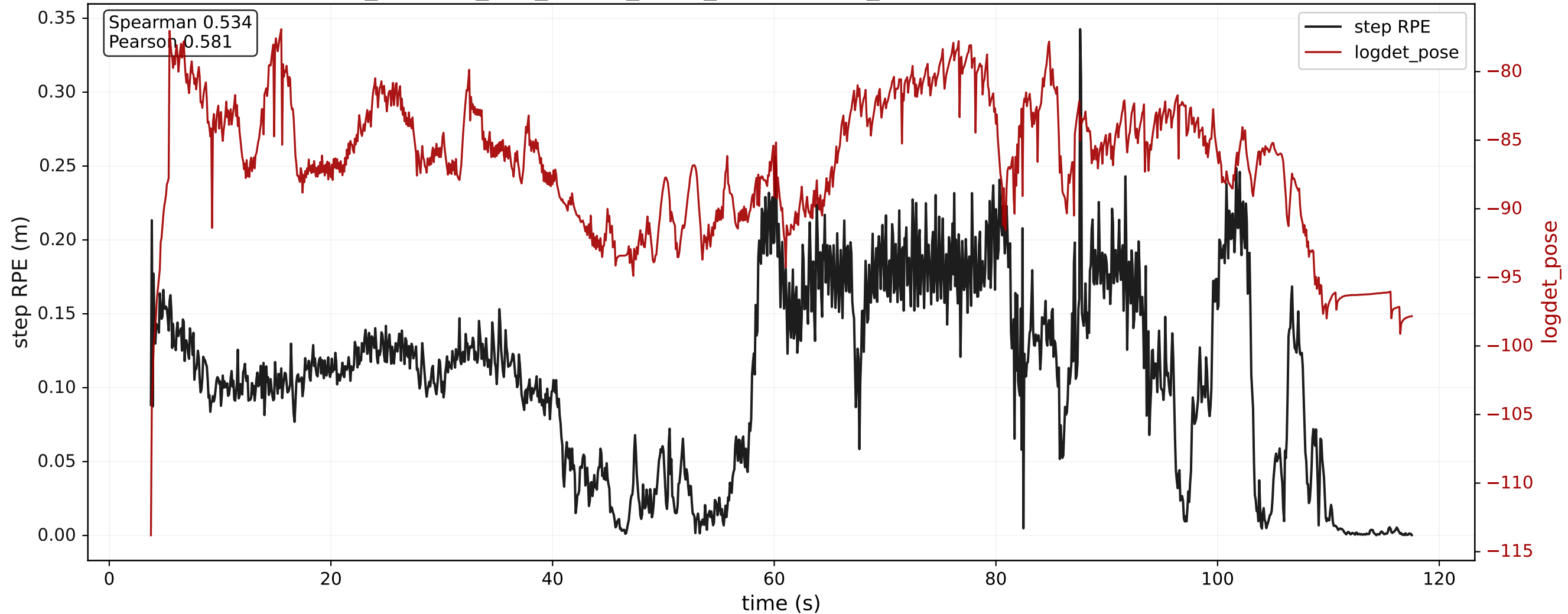
spot_outdoor_day_penno_short_loop: logdet_pose and Step-RPE over Time
