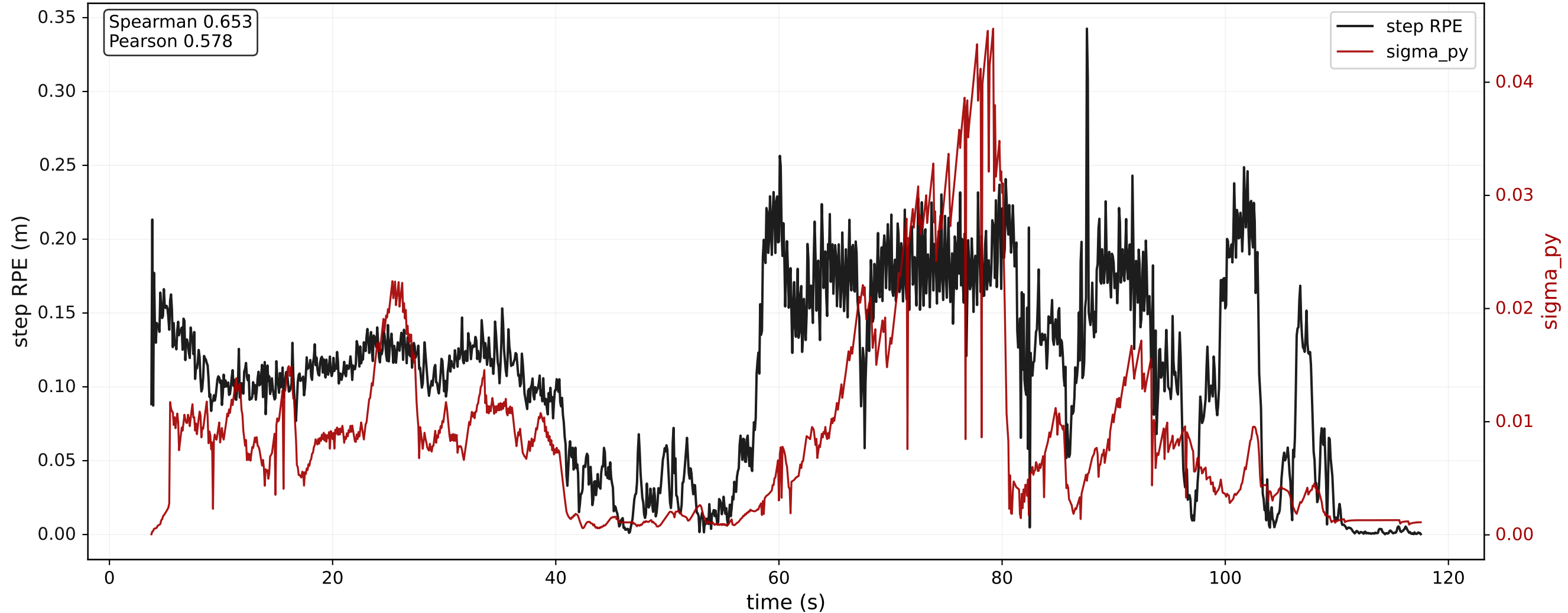
spot_outdoor_day_penno_short_loop: sigma_py and Step-RPE over Time
