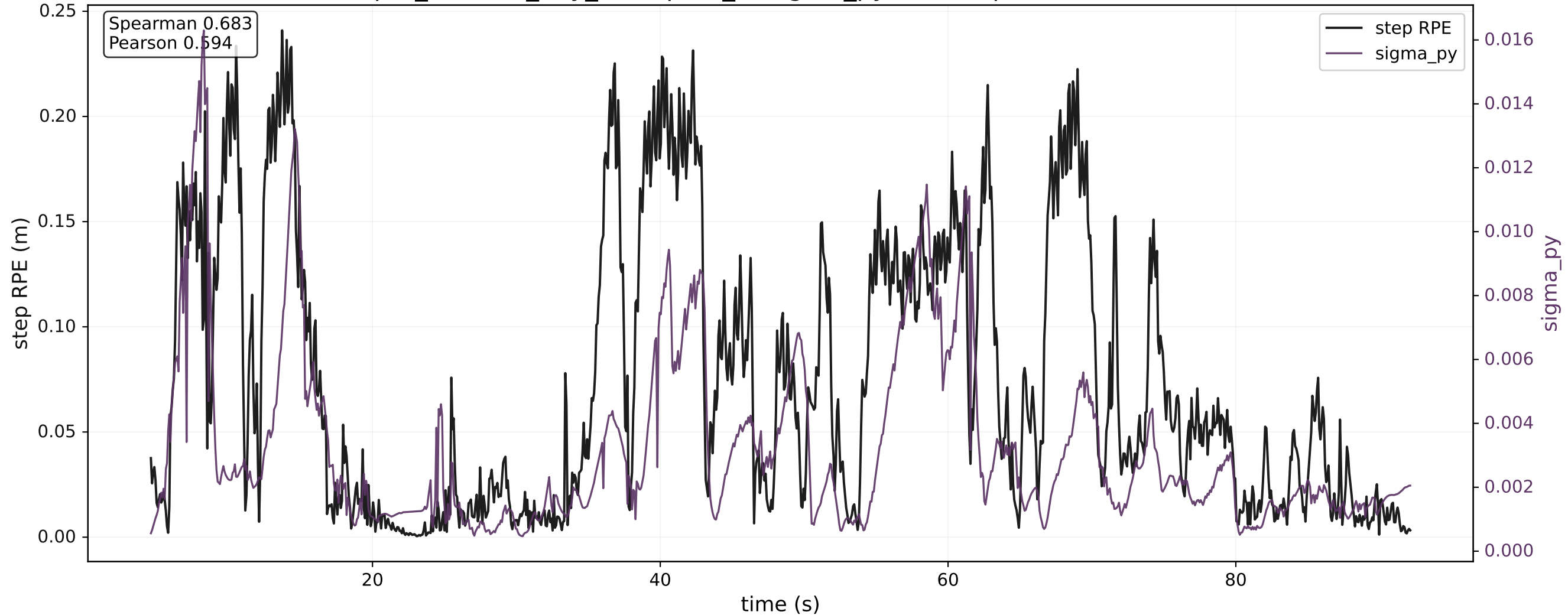
spot_outdoor_day_skatepark_1: sigma_py and Step-RPE over Time
