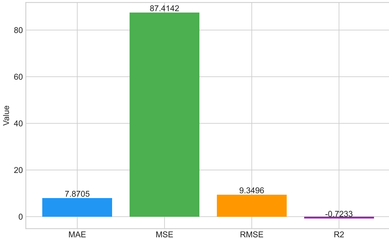
Evaluation Metrics
