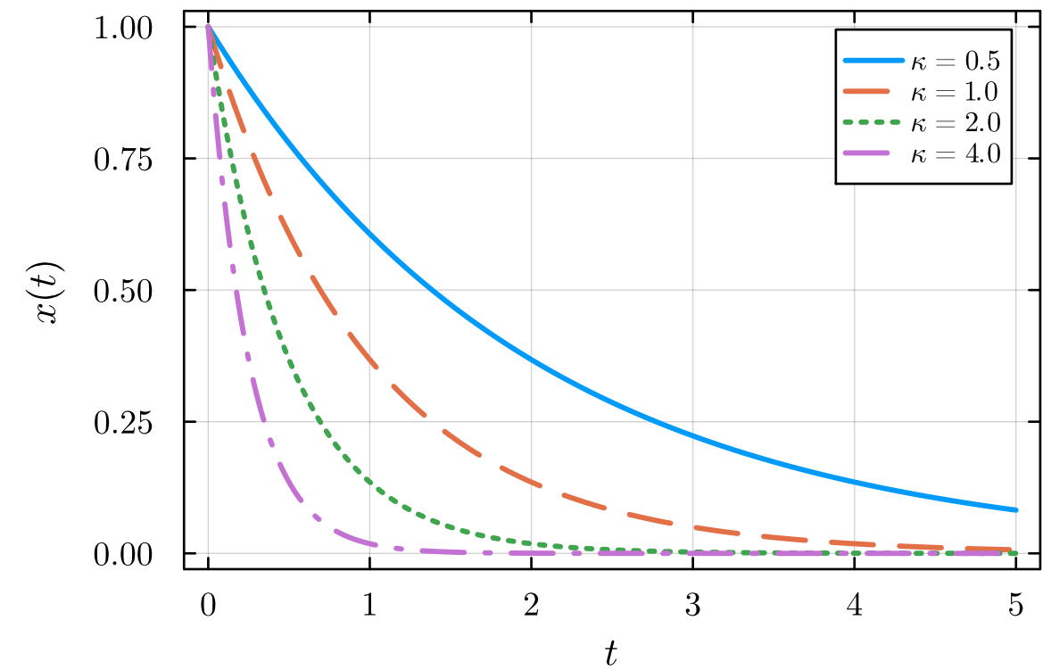
(C) \dot{x} = -\kappa x
