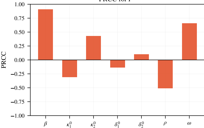
PRCC for I^*
