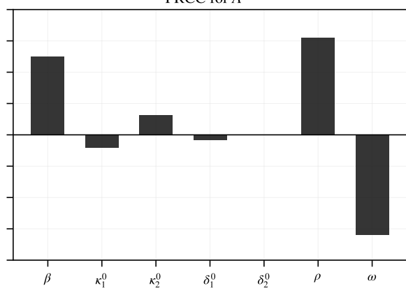
PRCC for A^*
