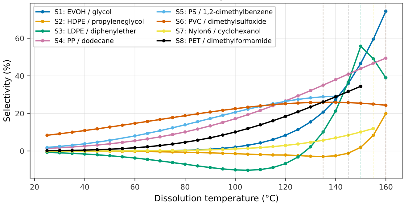
Per-step selectivity vs temperature
