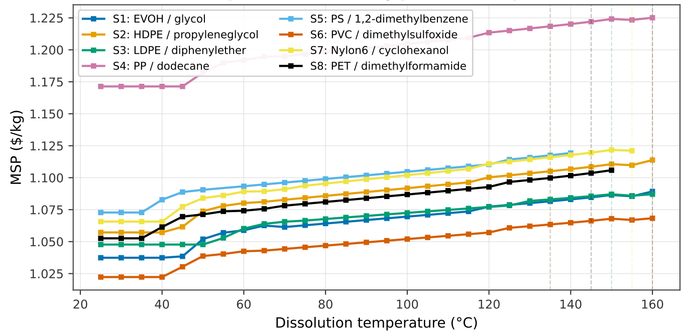
Per-step minimum selling price vs temperature
