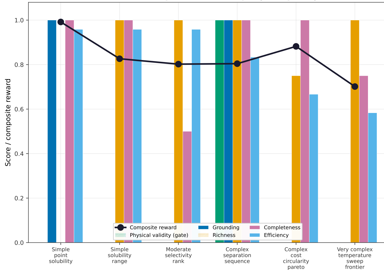
Reward decomposition across query complexity
