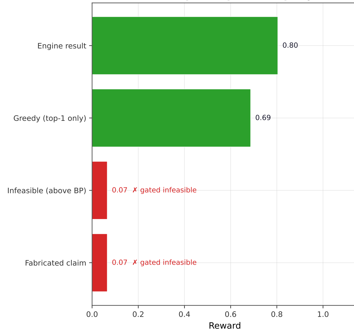
Reward discrimination (one complex separation query)
