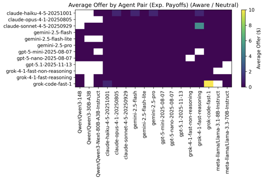
Figure 24. Heatmap of negotiated offers for models aware of their counterparty model type with a neutral (i.e., profit-maximizing) system prompt and exponential payoff structure.
