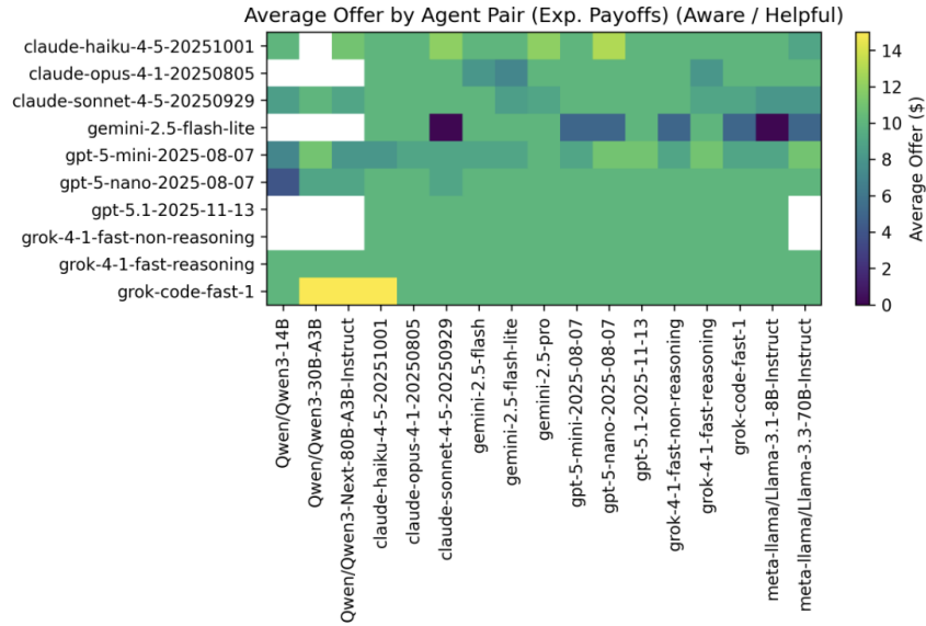
Figure 23. Heatmap of negotiated offers for models aware of their counterparty model type with a helpful system prompt and exponential payoff structure.
