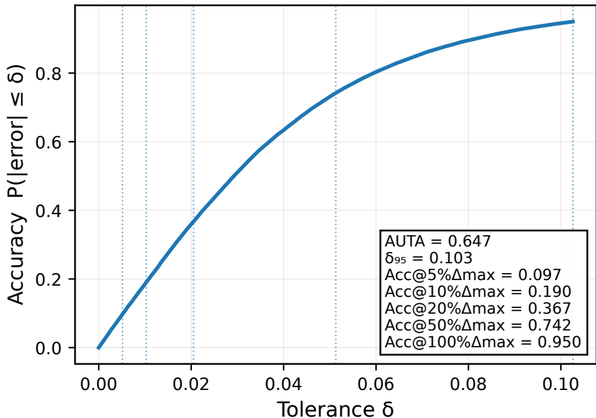
Tolerance-Accuracy Curve
