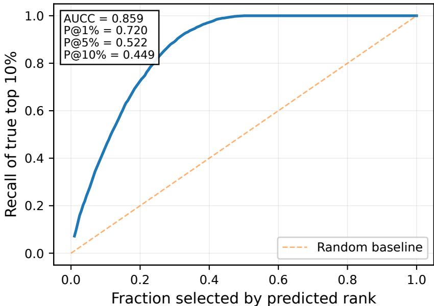
Top-k Capture Curve
