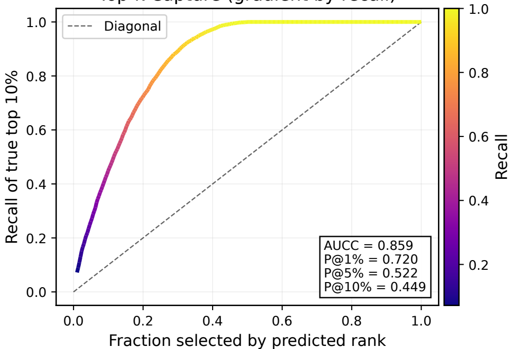
Top-k Capture (gradient by recall)
