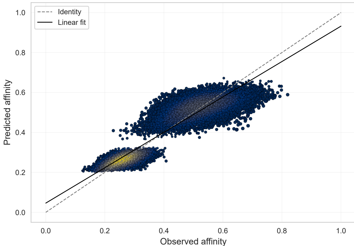
Predicted vs Observed ( R^2=0.884 ; r=0.940 ) — covidis
