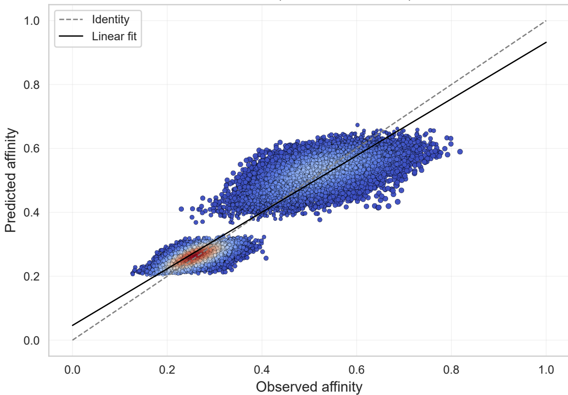
Predicted vs Observed ( R^2=0.884 ; r=0.940 ) — coolwarm
