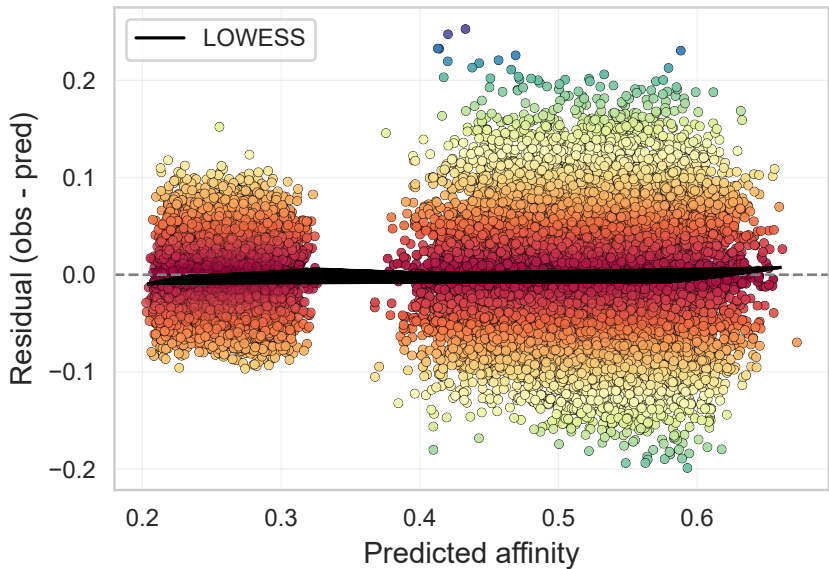
Residuals vs Predicted — Spectral
