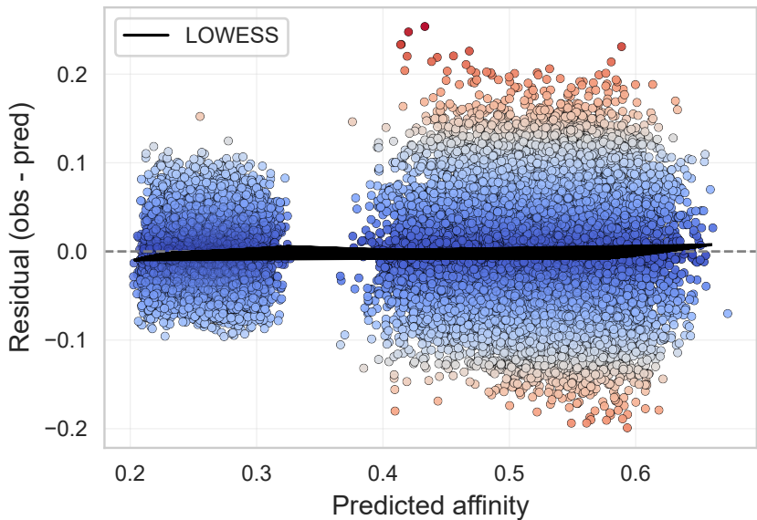
Residuals vs Predicted — coolwarm
