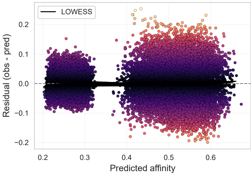
Residuals vs Predicted — magma
