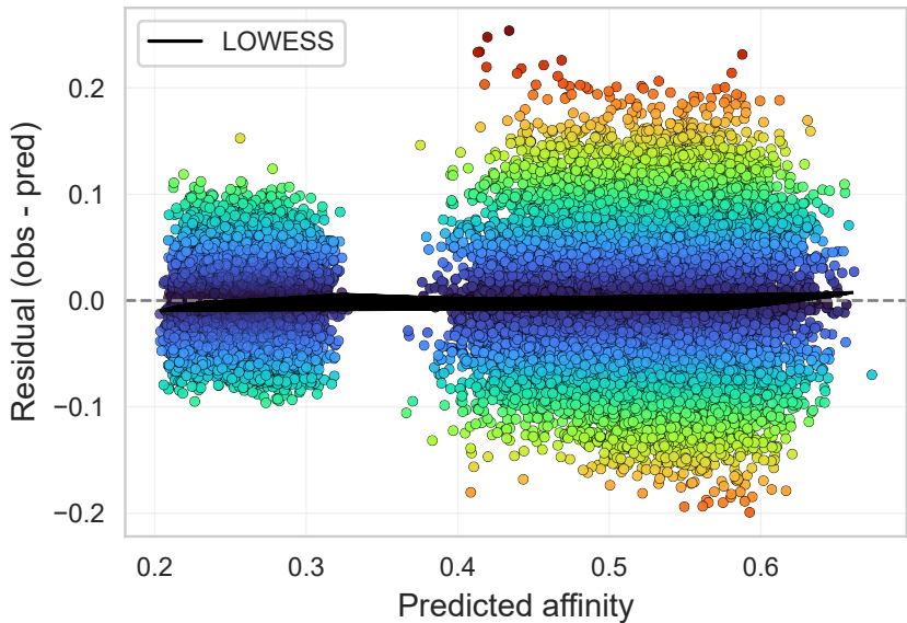
Residuals vs Predicted — turbo
