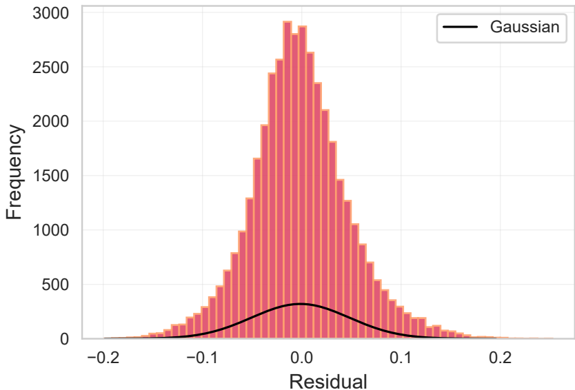
Distribution of residuals — magma
