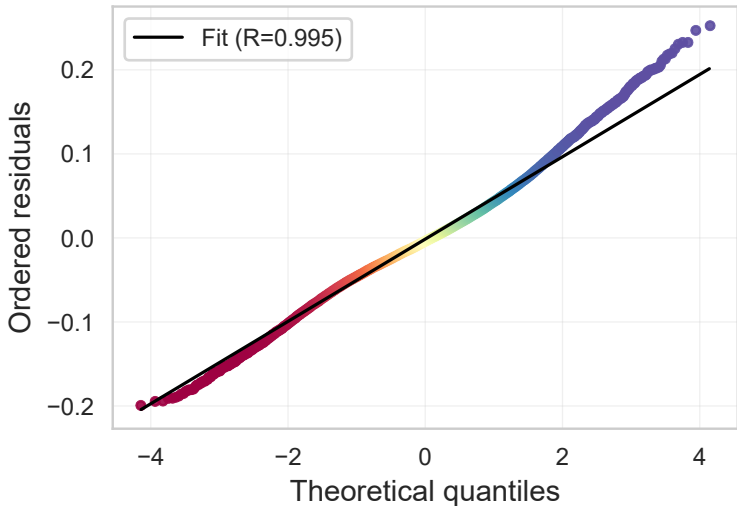
Q-Q plot of residuals — Spectral
