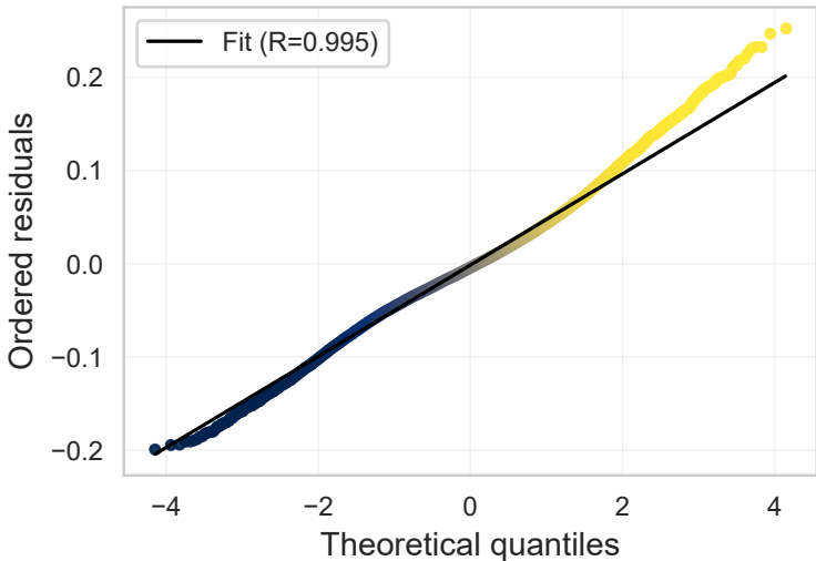
Q-Q plot of residuals — covidis
