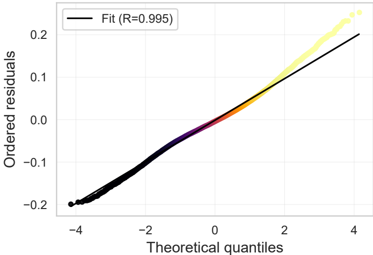
Q-Q plot of residuals — inferno
