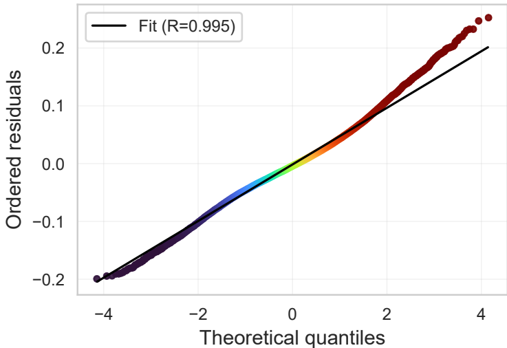
Q-Q plot of residuals — turbo
