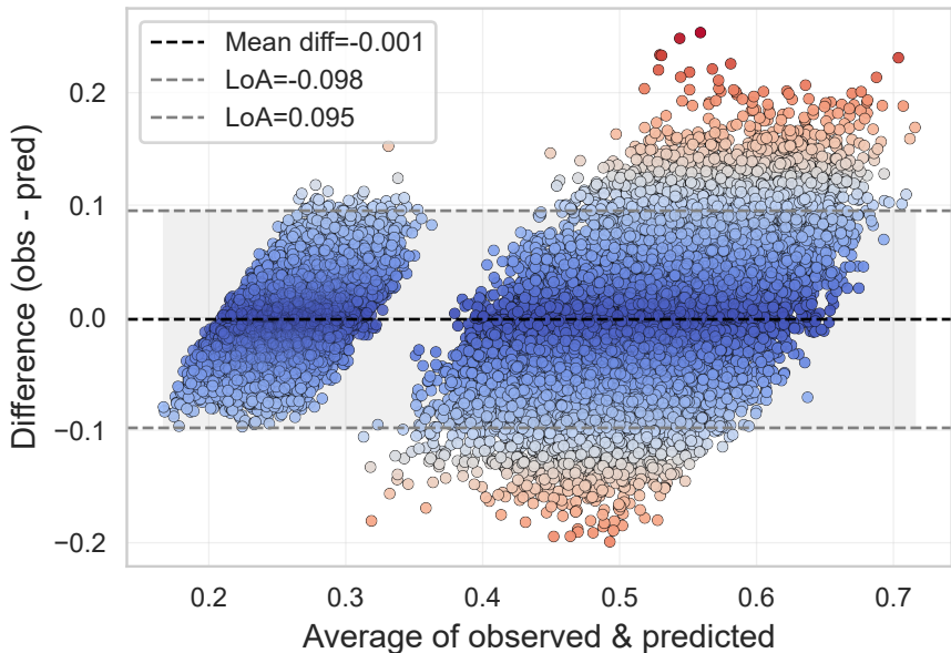
Bland–Altman (outside LoA: 6.1%) — coolwarm
