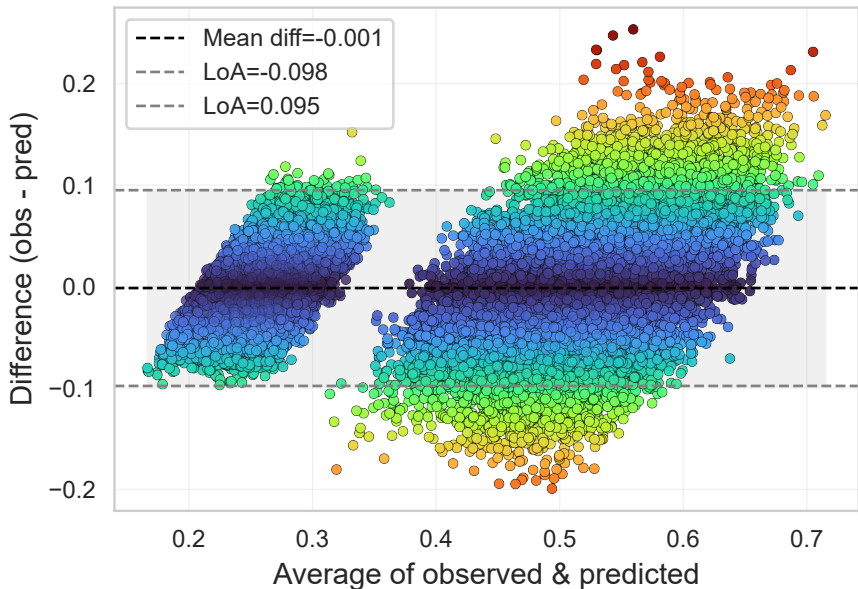
Bland–Altman (outside LoA: 6.1%) — turbo
