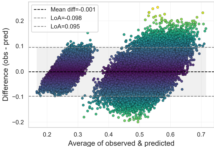
Bland–Altman (outside LoA: 6.1%) — viridis
