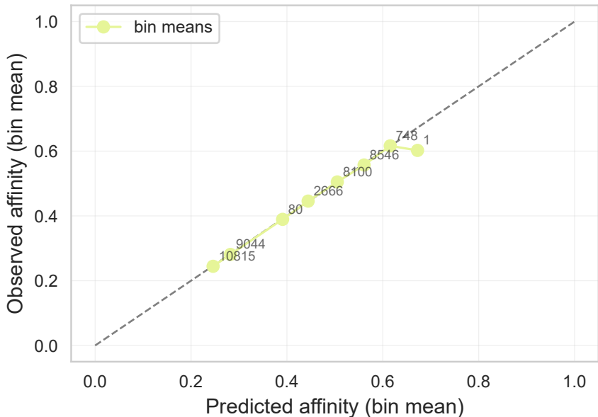
Reliability (ECE=0.002, MCE=0.070) — Spectral
