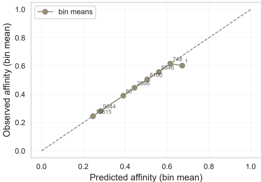
Reliability (ECE=0.002, MCE=0.070) — covidis
