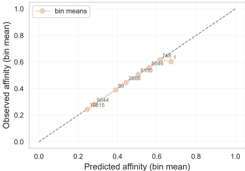
Reliability (ECE=0.002, MCE=0.070) — coolwarm
