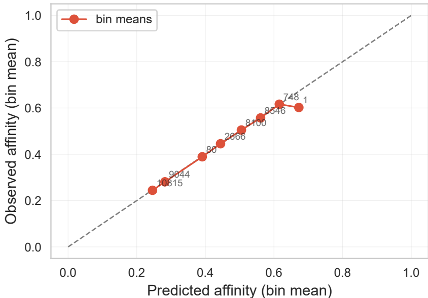
Reliability (ECE=0.002, MCE=0.070) — inferno
