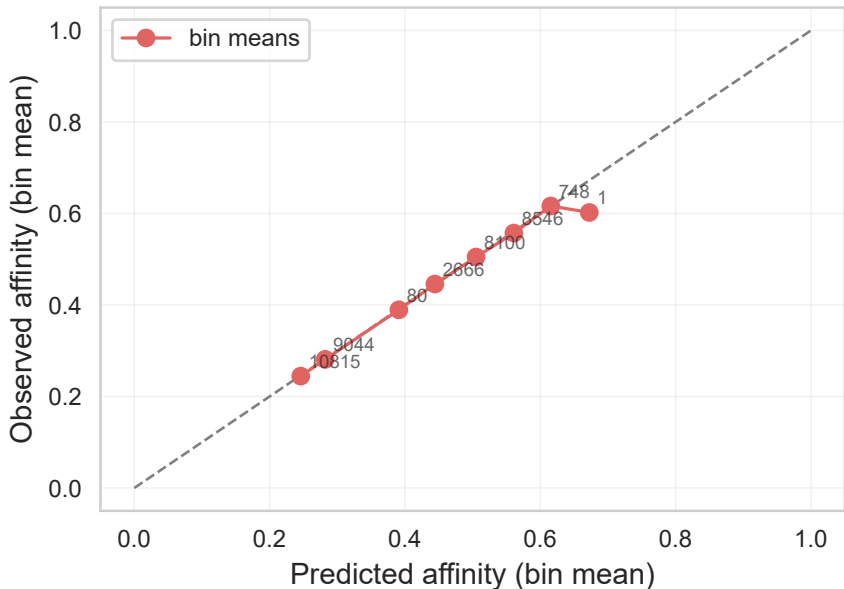
Reliability (ECE=0.002, MCE=0.070) — plasma
