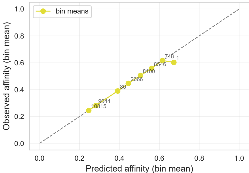
Reliability (ECE=0.002, MCE=0.070) — turbo
