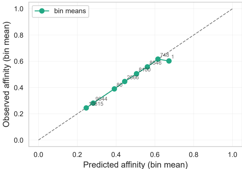
Reliability (ECE=0.002, MCE=0.070) — viridis
