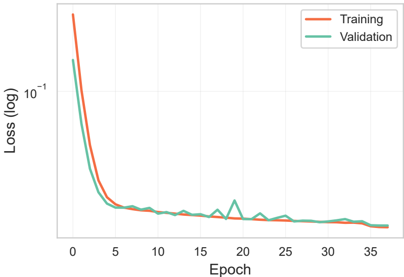
Model loss over epochs — Spectral
