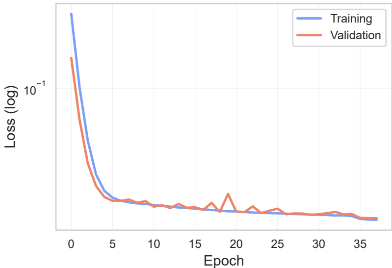
Model loss over epochs — coolwarm
