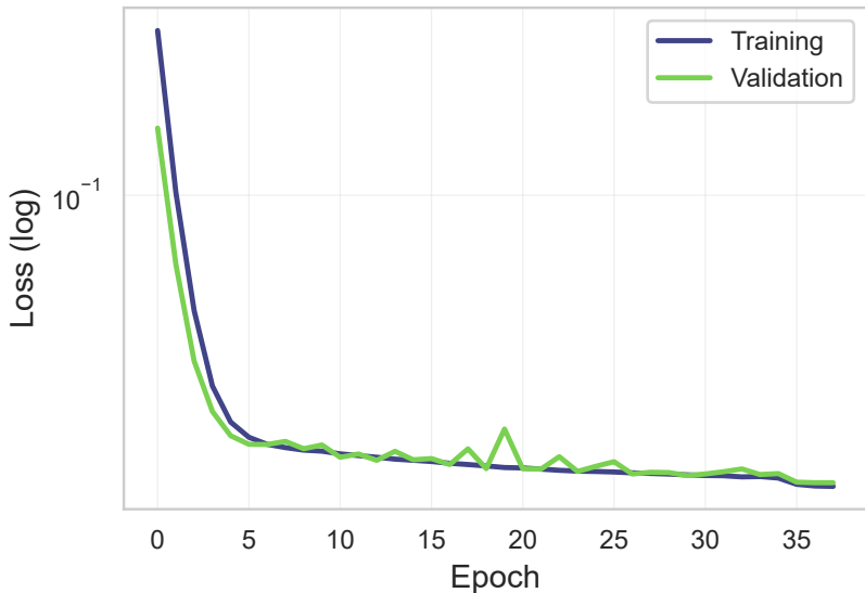
Model loss over epochs — viridis
