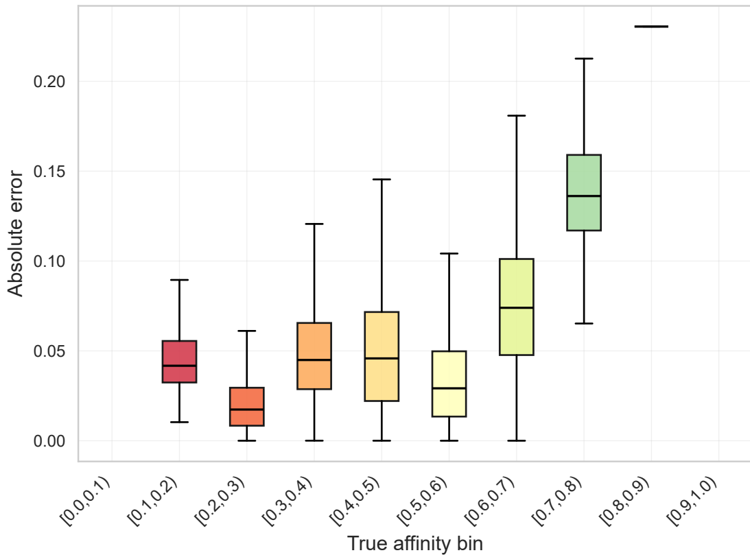
Absolute prediction error by true-affinity bins — Spectral
