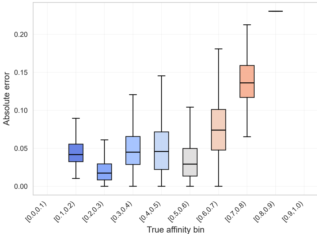
Absolute prediction error by true-affinity bins — coolwarm
