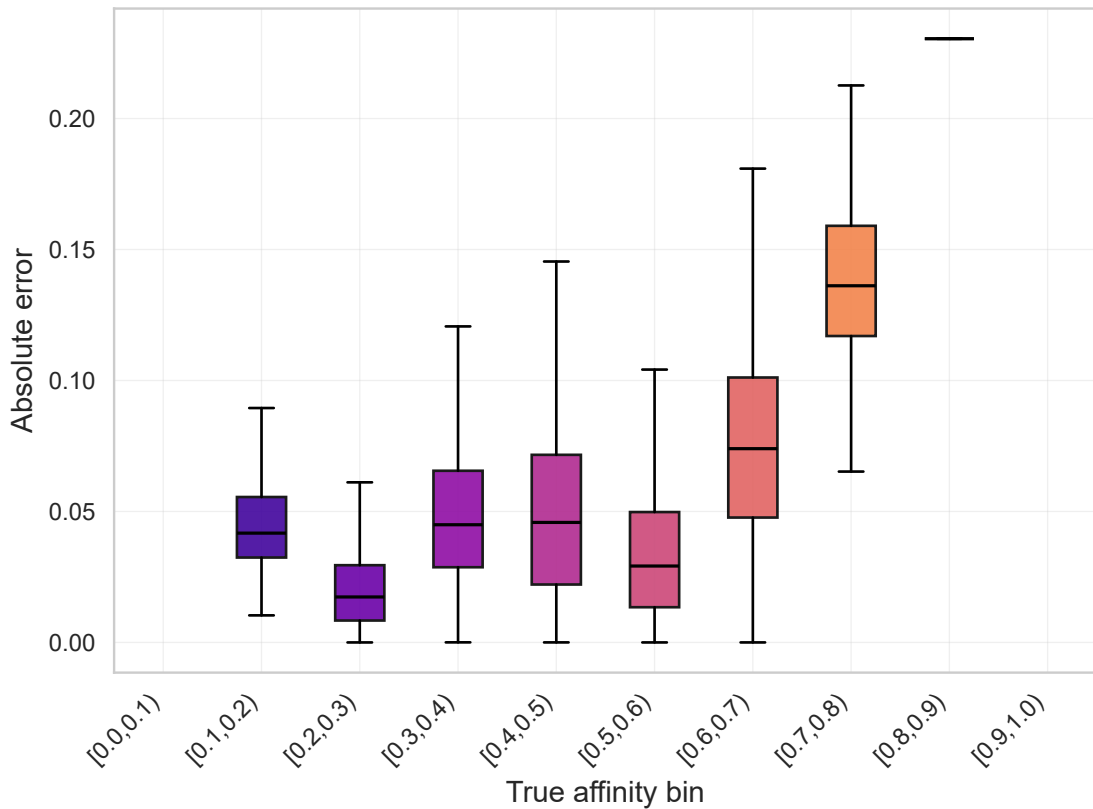
Absolute prediction error by true-affinity bins — plasma
