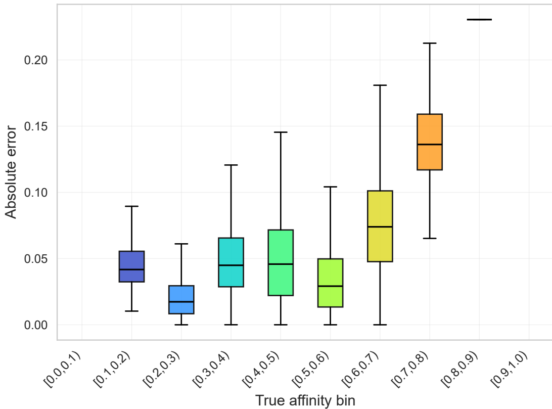
Absolute prediction error by true-affinity bins — turbo
