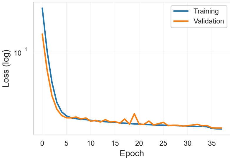
Model loss over epochs
